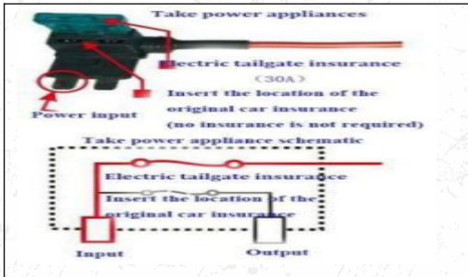
13. Fuse definition diagram
