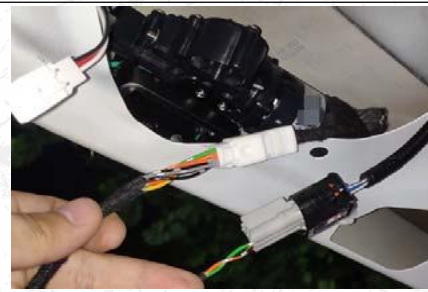
14. Unplug the original lock block wiring harness and insert our wiring harness
